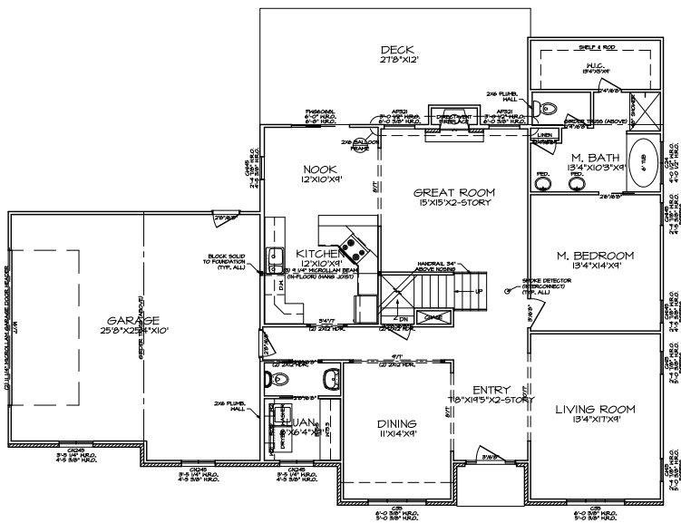
FIRST FLOOR PLAN A-4 SCALE: 1/4"=1'-0"
