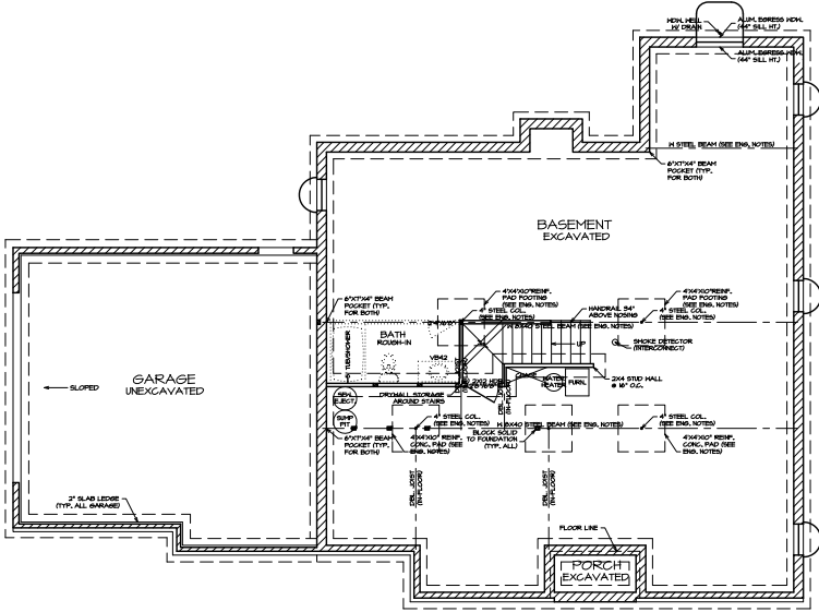
FOUNDATION PLAN A-3 SCALE: 1/4"=1'-0"
